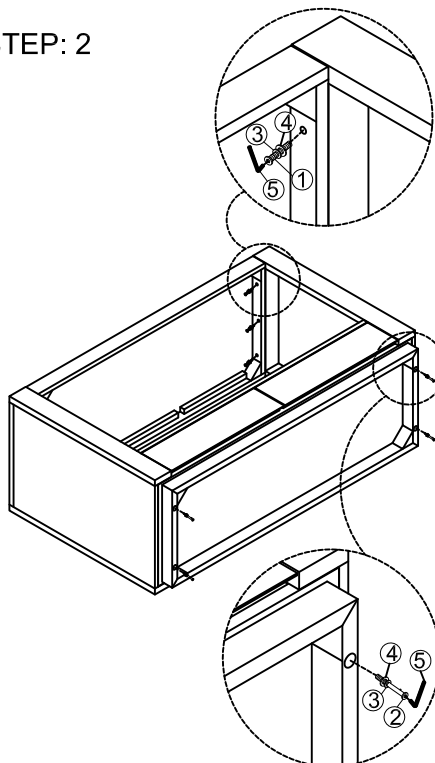
Assembly Completed
